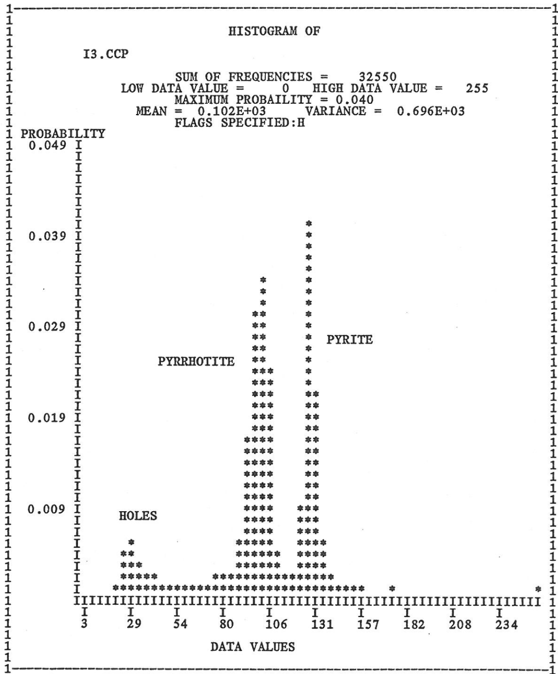
Figure 7 illustrates the histogram of mineralogical content of image in Figure 1 in terms of reflectance.
