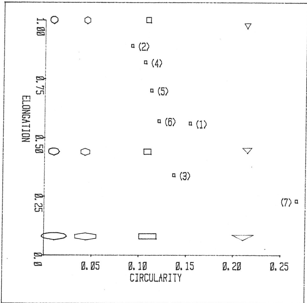
Figure 6 shows the circularity and elongation measures for ideal and real figures. The real figures correspond to the numbered grains of Figure 1.
