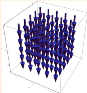
(b) Result Of The Curl Operator
